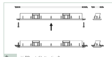
O viti TP autofilettanti ø 3 mm non comprese BH auto - threading screws ø 3 mm are not included
